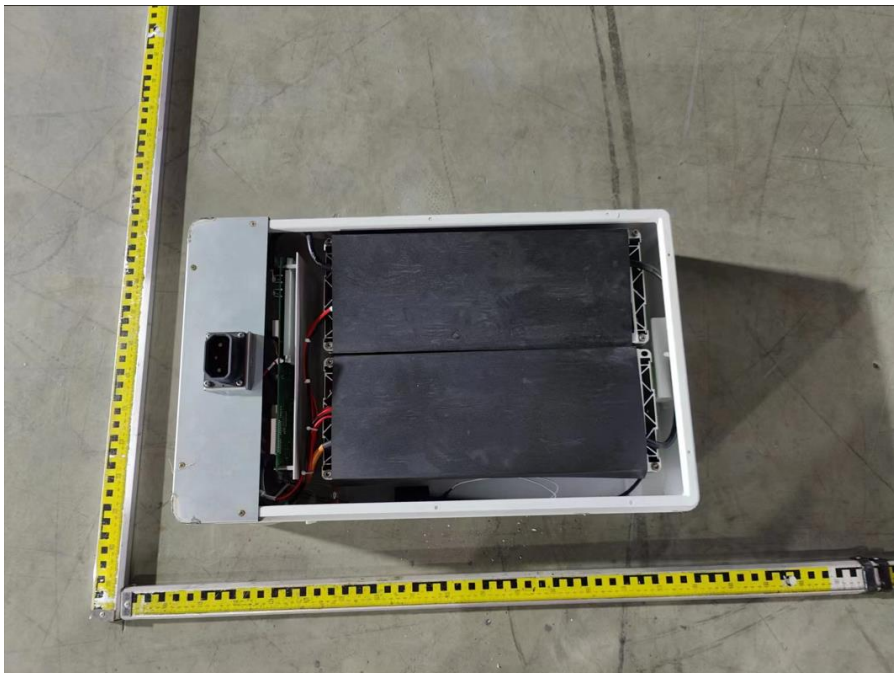
Internal view of BYES-5000 battery box
